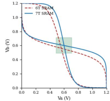
Fig. 5 Static Noise Margin (SNM) comparison using butterfly curves
